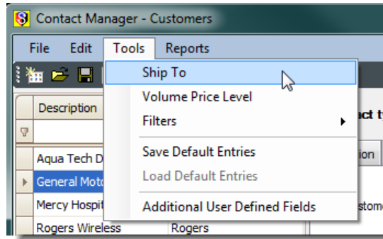
Figure 22: Tools menu
